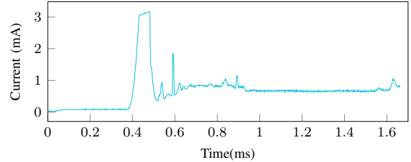
Fig. 5. Current consumption during hardware boot.
