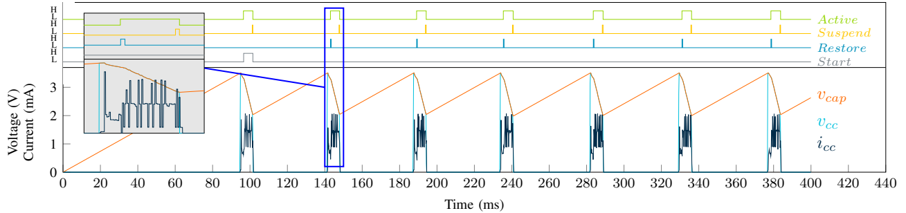
Fig. 9. Simulation trace of a reactive intermittent computing system powered by a 200\mu\text{A} current-limited power supply. The top traces show the logic levels of GPIO pins indicating the operation of the device, and the lower traces show the microcontroller supply voltage ( v_{cc} ), the storage capacitor voltage ( v_{cap} ) and the current draw ( i_{cc} ).
